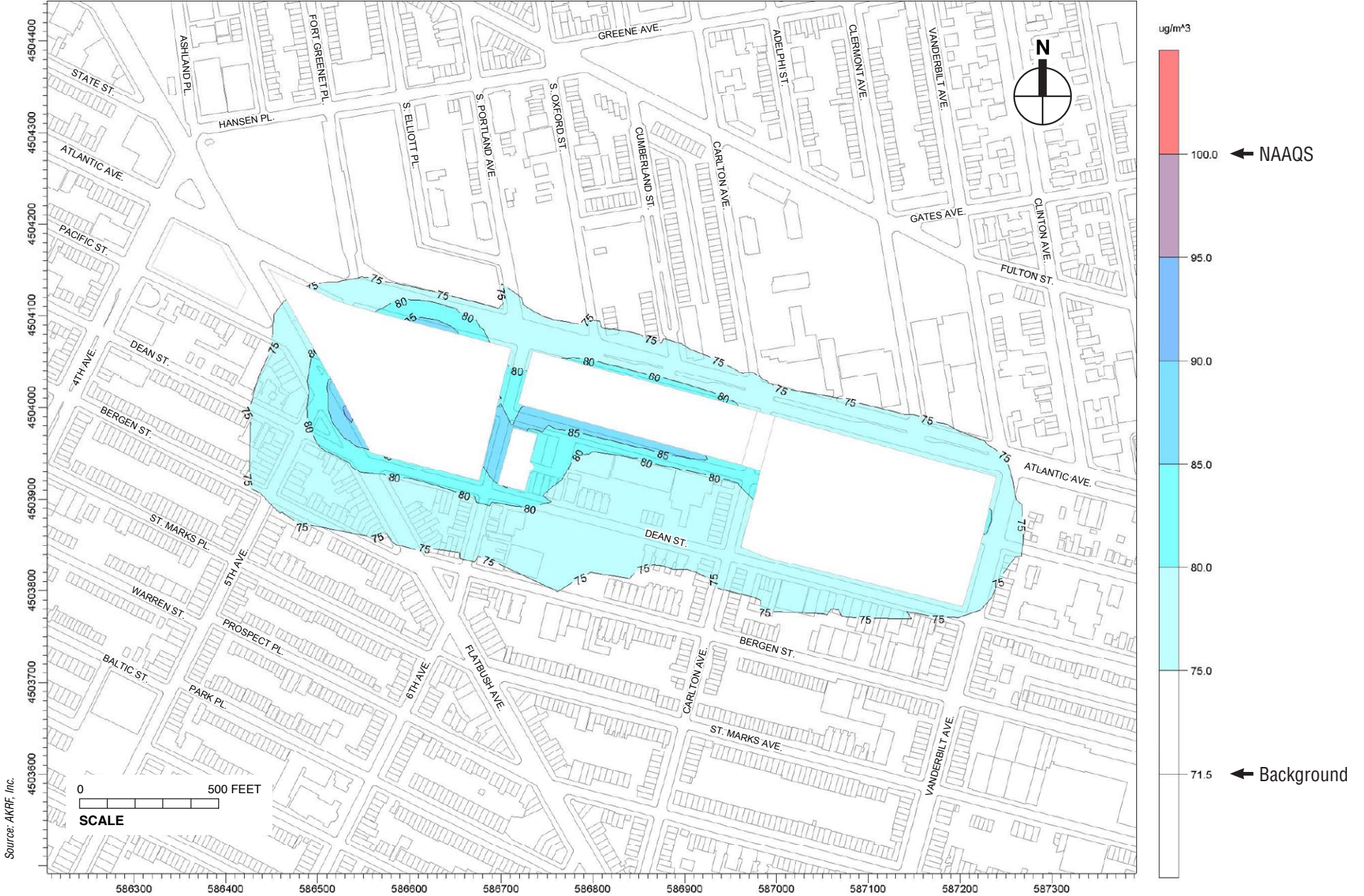
Total Maximum Predicted Annual Average NO 2 Concentration Construction Scenario A1
