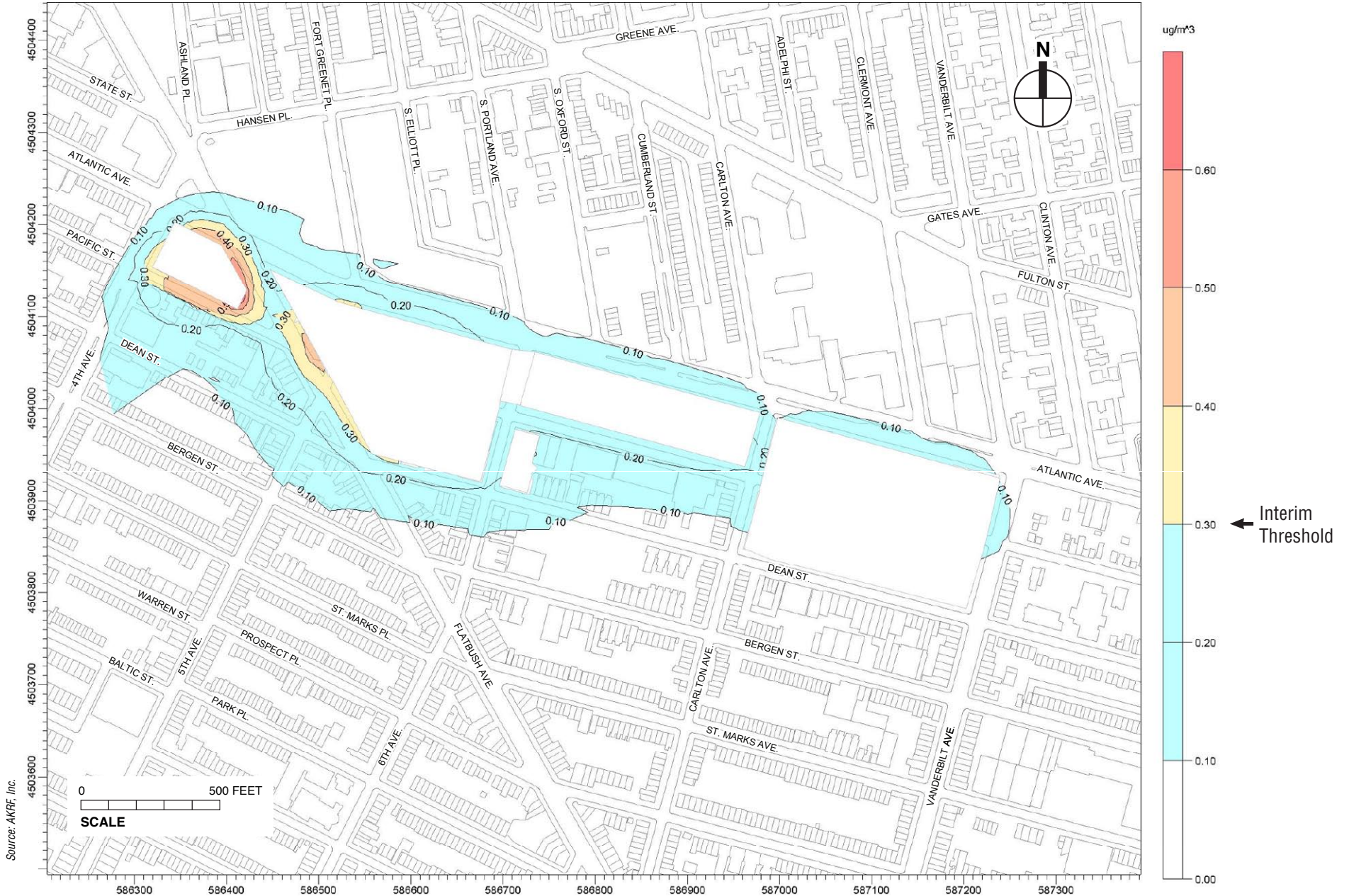
Maximum Predicted Annual Average Increase in PM 2.5 Concentration Construction Scenario A2
