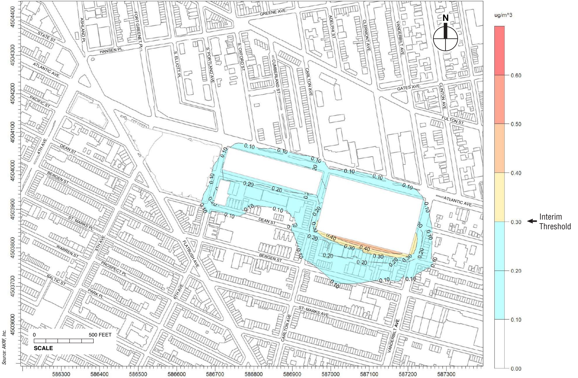
Maximum Predicted Annual Average Increase in PM 2.5 Concentration Construction Scenario A4
